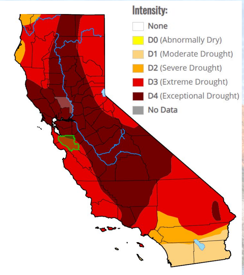
U.S. Drought Monitor, 10/19/21
