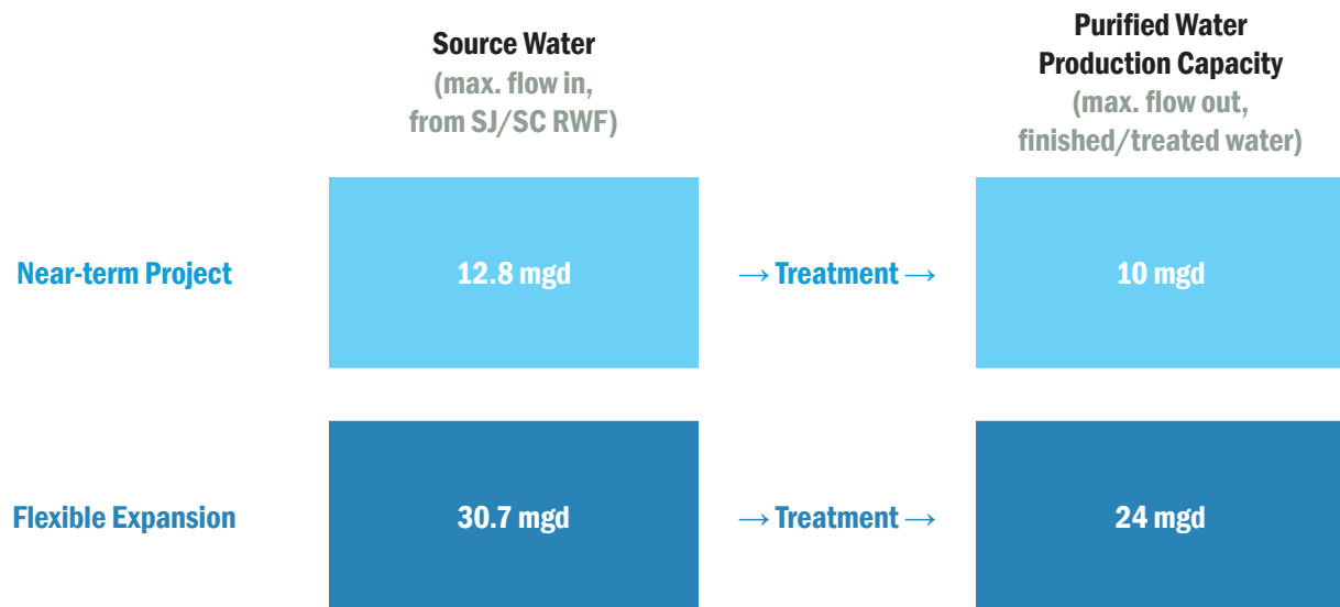
Figure 9-2. Assumed source water flow rates and production capacities for flex implementation of a San José-based AWWP
