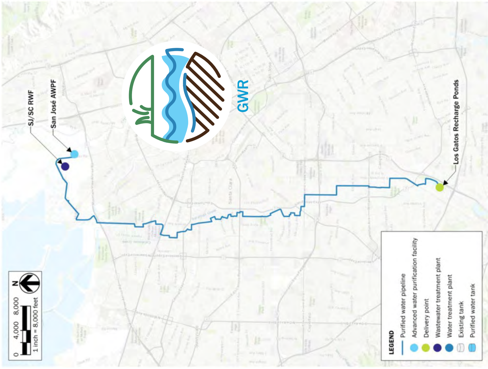
Figure 6-1. Portfolio 1a: SJ GWR facility locations and pipeline alignments
