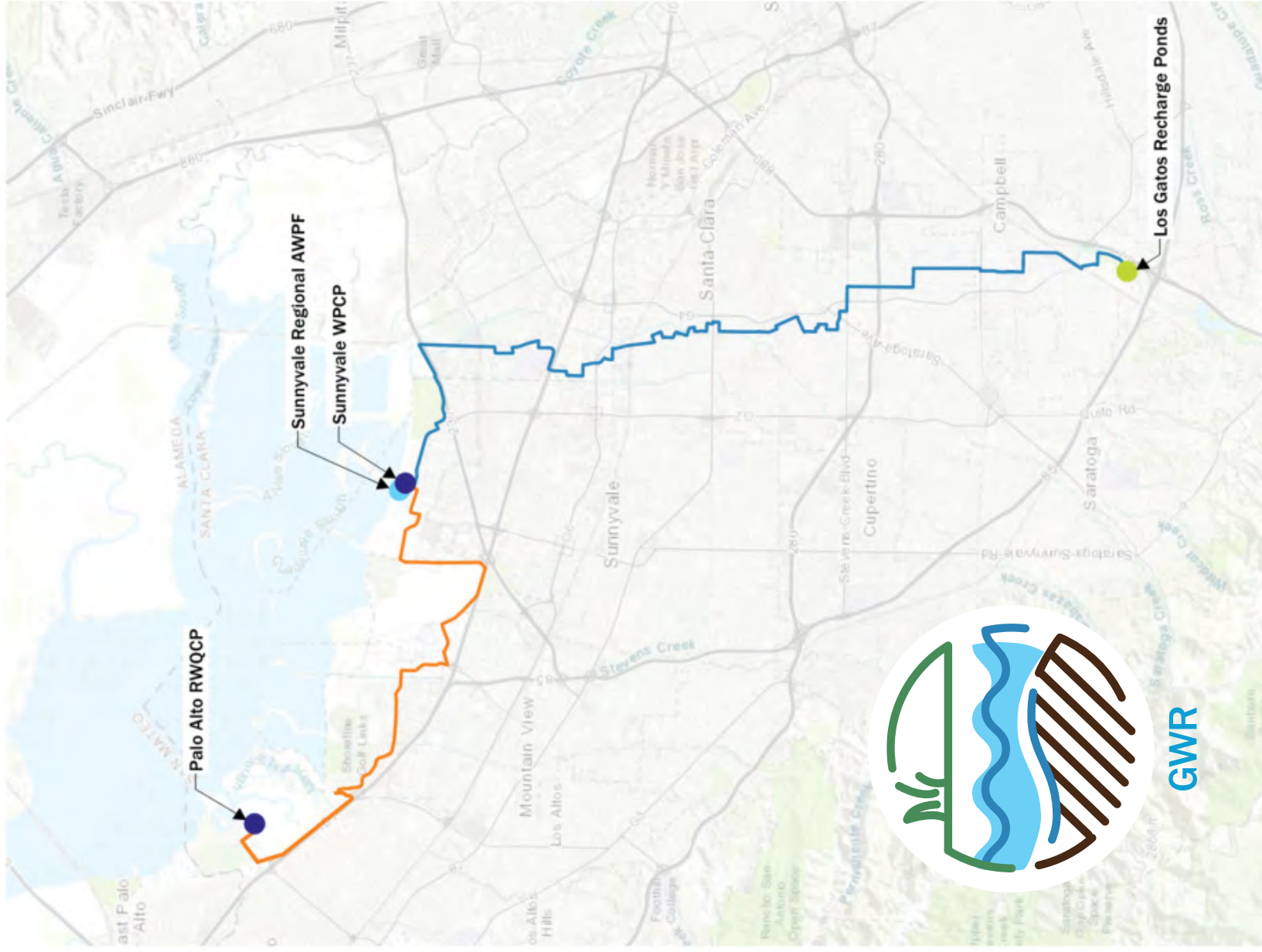
Figure 6-5. Portfolio 2a: PA (+SV) GWR facility locations and pipeline alignments
